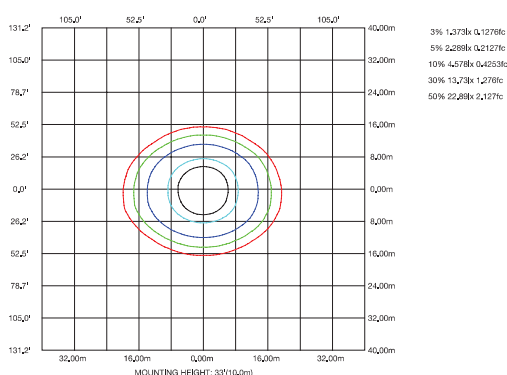
ISOLUX DIAGRAM
