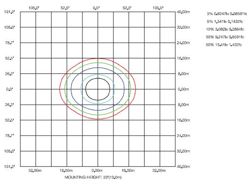
ISOLUX DIAGRAM
