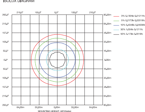
ISOLUX DIAGRAM
