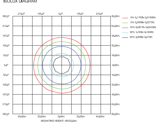
ISOLUX DIAGRAM
