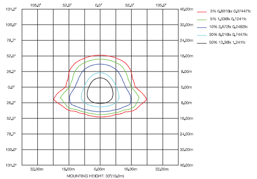
ISOLUX DIAGRAM
