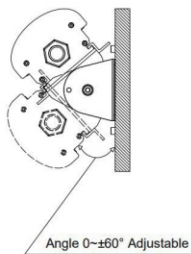
D.Wall mounting
