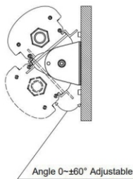
D.Wall mounting
