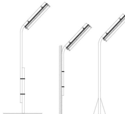
E.Pole Mounting
