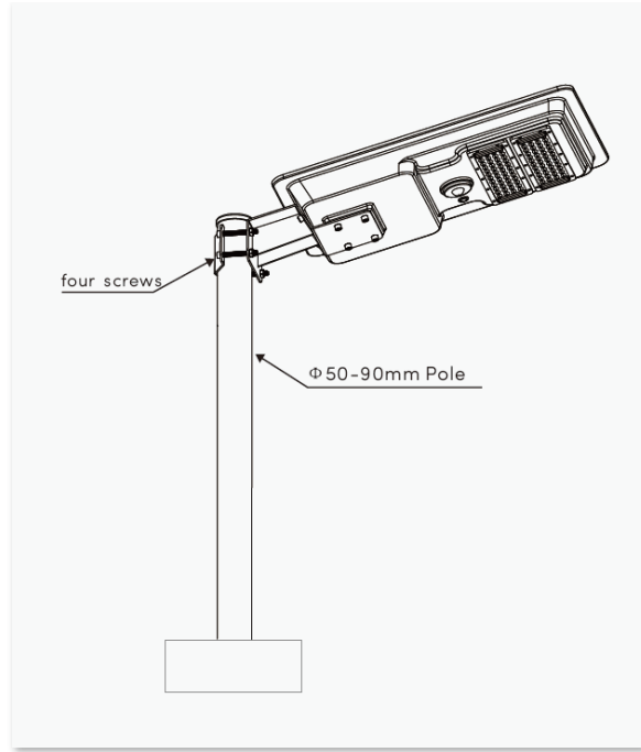
2.Bracket Mounting
