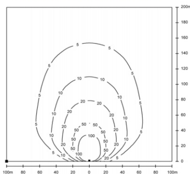
4x150W-DC48V 9m Isolux curve
