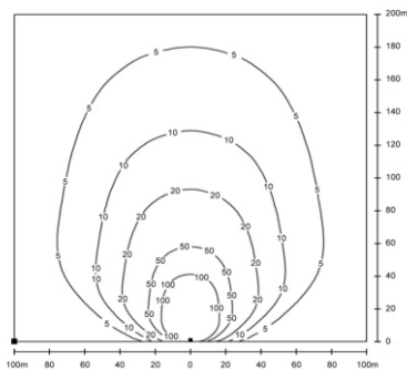
4×200W-DC48V 9m Isolux curve
