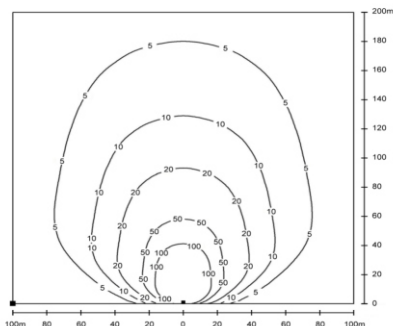
4x200W-DC48V 9m Isolux curve
