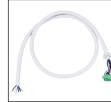
WSD-OL-6CPC-6FT-W Six-core Power Cord Length: 6FT Note:Emergency Battery backup Inputs required (2FT,4FT,8FT)
