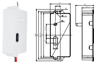
BRI810-B-D Microwave Motion Sensor
