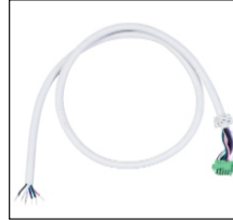
WSD-OL-6CPC-W Six-core Power Cord Length: 47.83 inch Note:Emergency Battery backup Inputs required (2FT,4FT,8FT)
