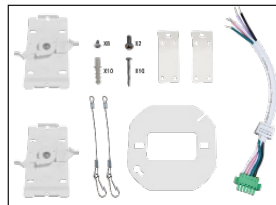
WSD-OL-SMK-WMK-W Wall and Surface Mounting KIT Wire Rope Length:Y0.04X4.7 inch (2PCS) Wire Length : 7.87 inch (2FT,4FT,8FT)
