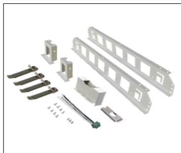
WSD-2FT-OL-RMK-G2 Recessed Mounting Kit For 2FT Architecture Selectable LED Linear Light
