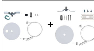
WSD-OL-CIK-A2 Ceiling Install KIT Wire Rope Length:Y0.06X39.4 inch(2PCS) (2FT,4FT,8FT)
