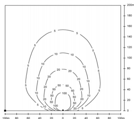
4×150W-DC48V 9m Isolux curve
