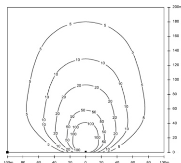
4x200W-DC48V 9m Isolux curve
